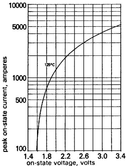
Figure 16 Limit on-state characteristic
