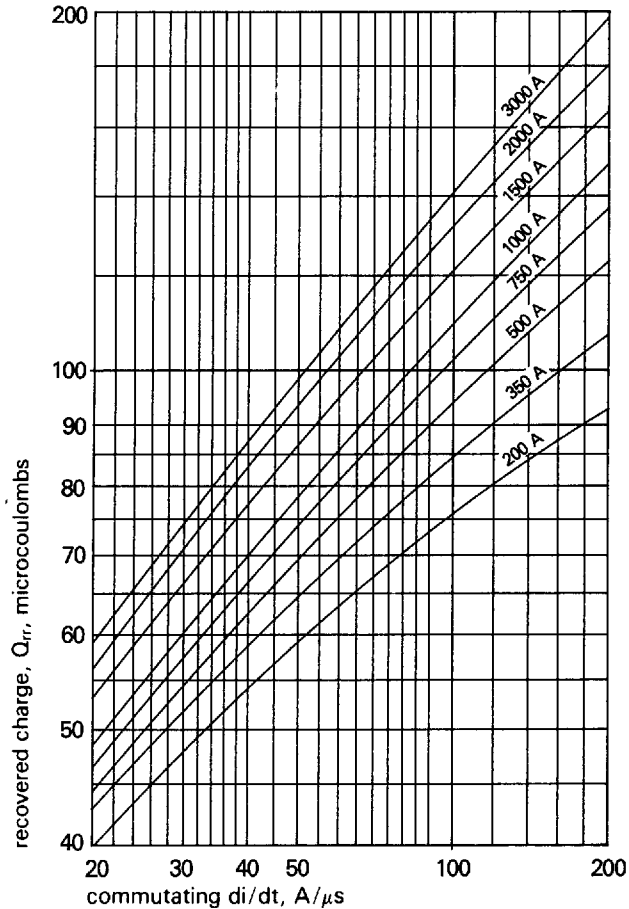
Figure 11 Maximum recovered charge at 125°C junction temperature
